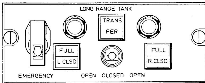
CONTROL PANEL ( CENTER CONSOLE INSTALLATION )
