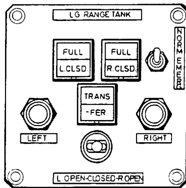
CONTROL PANEL ( INSTRUMENT PANEL INSTALLATION )
